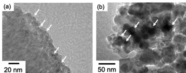
Fig. 9 Transmission electron microscopy (TEM) images of (a) Ir(CN) 2 -Ni/SiO 2 -Al 2 O 3 -0.2 and (b) Ir(CN) 2 -Ni/TiO 2 -0.20. The white arrows indicate the Ir–Ni alloy particles.
