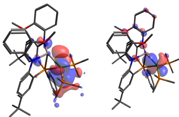
Fig. 5 Pictorial representation of HOMO (left) and HOMO (–6) (right) of 2\text{-(PMe}_3)_2 . Isosurface value set to 0.03 \text{ e A}^{-3} . Hydrogen atoms are omitted for clarity.
