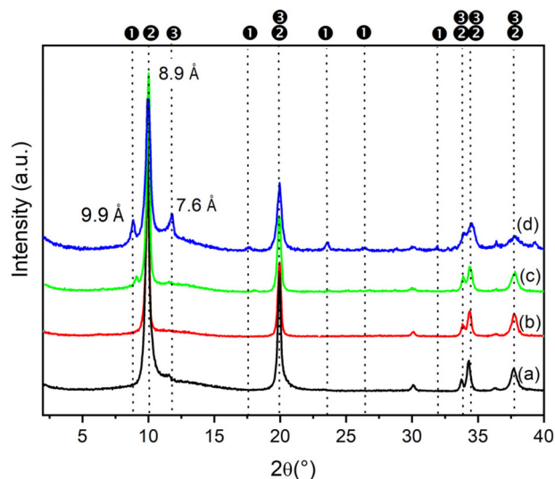
Fig. 1 PXRD patterns of ZnAl LDH synthesized by using \text{Zn(NO}_3)_2 \cdot 6\text{H}_2\text{O} and \text{Al(NO}_3)_3 \cdot 9\text{H}_2\text{O} salts with concentrations: 0.5 M (a); 1 M (b); 2 M and (c); 2.5 M (d). R = 1.2 , reaction time 48 h at a reflux temperature. ❶ \text{Zn}_5(\text{OH})_8(\text{NO}_3)_2 \cdot 2\text{H}_2\text{O} , ❷ \text{ZnAlNO}_3 , and ❸ \text{ZnAlCO}_3 .
