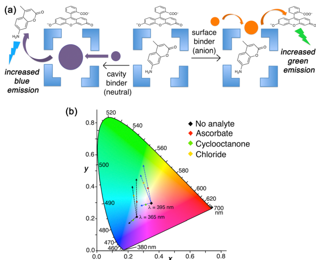
Fig. 11 (a) Cartoon representation of the dual fluorescence displacement assay used to probe cavity vs. surface binding of guest types in host H^W . (b) A CIE diagram showing the fluorescence colour changes associated with addition of (surface-binding) ascorbate, (cavity-binding) cyclooctanone, or chloride, to a mixture of H^W (150 \mu M), MAC (10 \mu M), FLU (20 \mu M) and Ru (30 \mu M). The two sets of dashed arrows starting at different starting points indicate the directions of colour shifts generated by different analytes using 365 nm (black arrows) or 395 nm excitation (blue arrows), respectively. These arrows are just to aid the eye: the end-points of each titration are illustrated by the coloured points.
