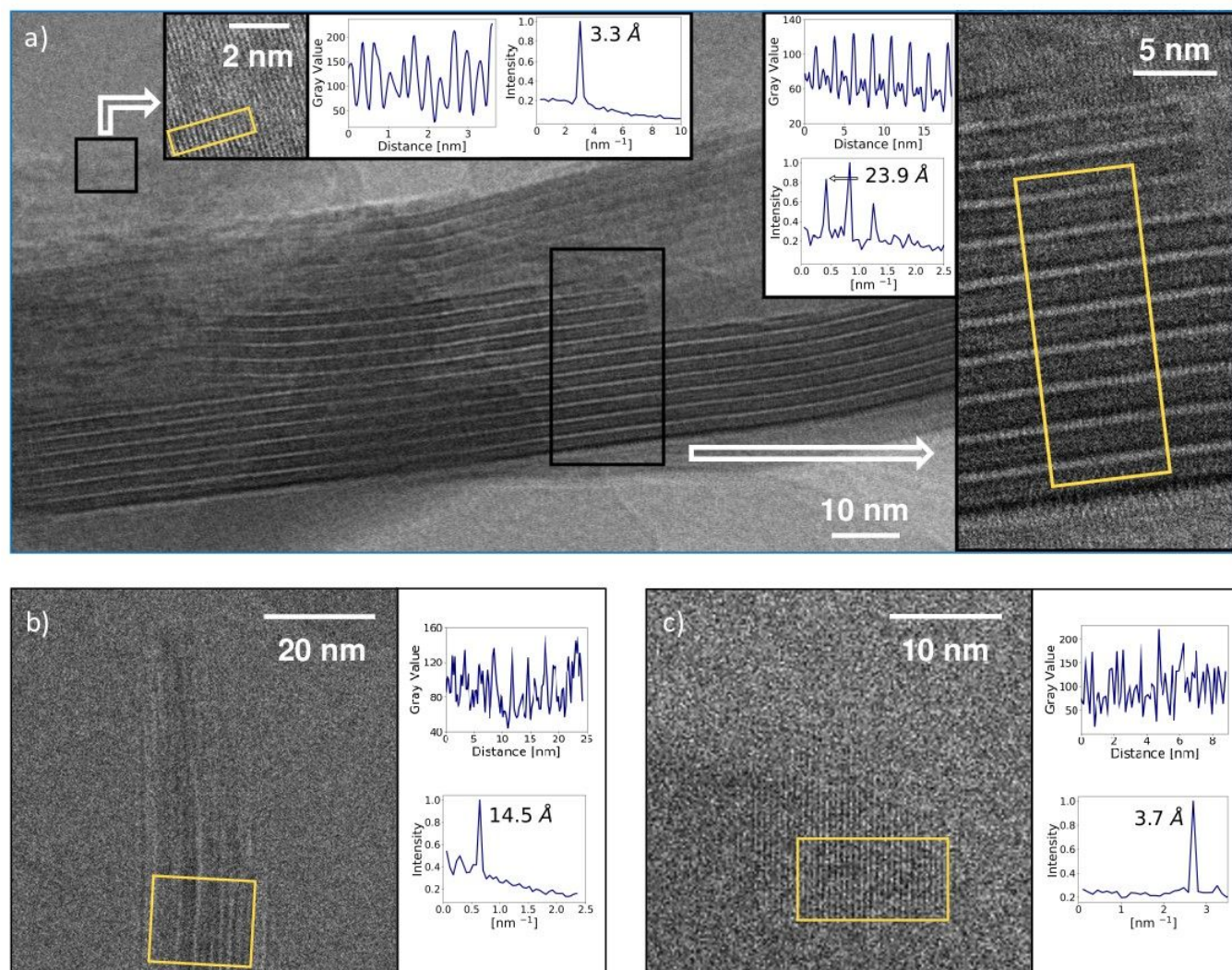
Fig. 3. (a) TEM images of M*HCA. The profiles were taken along long axes and averaging was performed along the short axes of the yellow rectangles. The inserts show the resulting profiles, their FFT, and the characteristic periodicity. (b), (c) Cryo-TEM images of MM*HCA. The analysis was performed similarly to (a).
