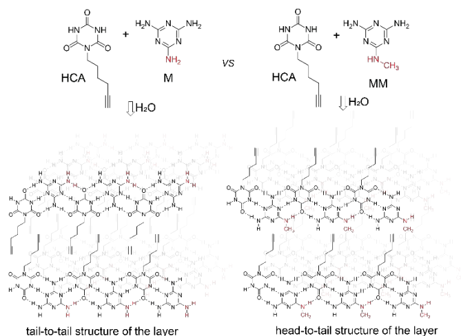
Fig. 1. Layered structures formed by self-assembly of hexynyl cyanuric acid with (a) melamine and (b) N-methylmelamine.
