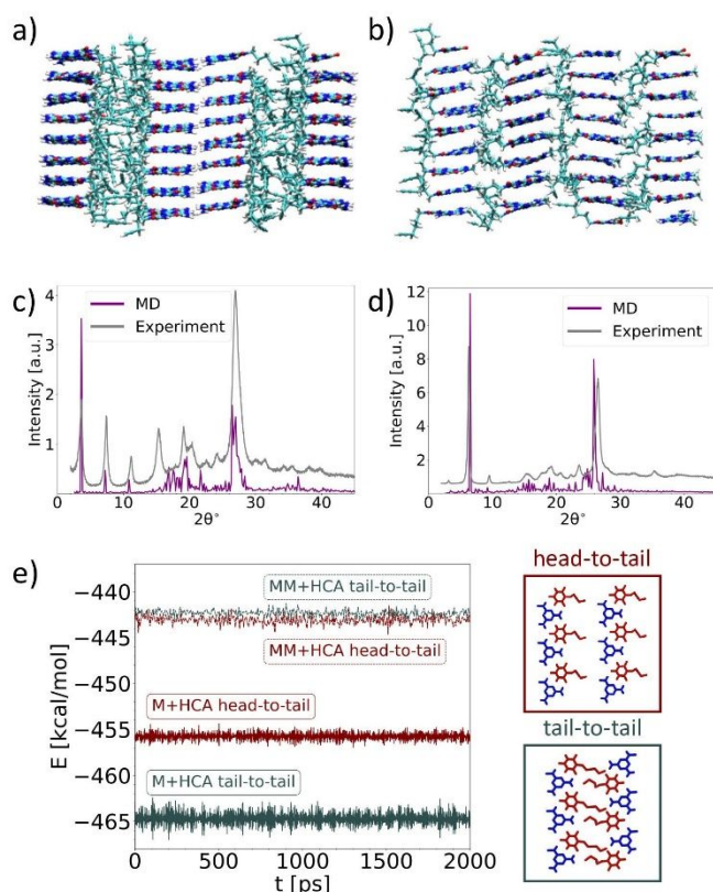
Fig. 4. Atomistic structures of (a) M*HCA and (b) MM*HCA obtained in MD simulations at T=300 K. (c),(d) Comparison of XRDs calculated from MD simulations with experimental XRDs. (e) Time evolution of the normalized potential energy of M*HCA (solid lines) and MM*HCA (dashed lines) systems with molecules arranged into two possible configurations: "head-to-tail" (red lines) and "tail-to-tail" (black lines).
