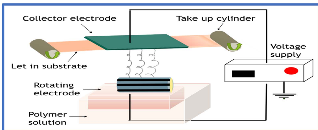
Fig. 5 Needleless electrospinning of polymeric solution.
