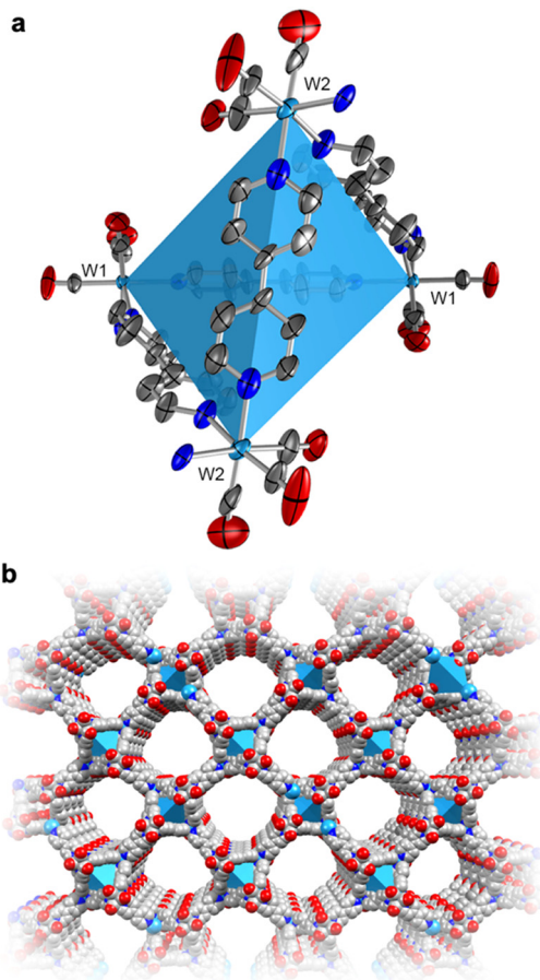
Fig. 1 (a) Room-temperature 3D-ED structure of the tetrahedral SBU, \{\text{W}(\text{CO})_3\text{-(bipy)}_{3/2}\}_4 , of W , showing the thermal displacement ellipsoids at 30% probability level. The coordination sphere is completed by half a bipy for each W center (with the N atom depicted). (b) The crystal structure of a single polymeric network of W as viewed down the crystallographic c axis (cf. Fig. S3, ESI†). H-atoms and the three identical, interpenetrated networks have been omitted for clarity. Color codes: W , light blue; O , red; N blue; C , grey.
