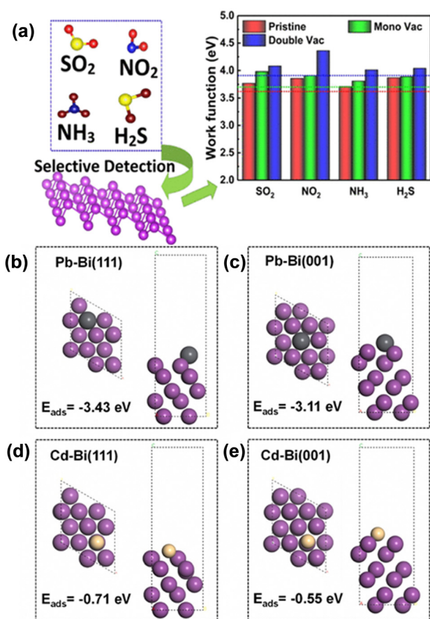
Fig. 7 (a) Sensing of SO 2 , NO 2 , NH 3 , and H 2 S gas using bismuthene. Reprinted with permission from ACS. 85 Adsorption energies and adsorption configurations of lead on (b) Bi-ene and bismuth nanosheets (c) and cadmium on Bi-ene (d) and (e) bismuth nanosheets, respectively (black, yellow and violet balls represent Pb, Cd and Bi atoms, respectively). Reprinted with permission from Elsevier. 86
