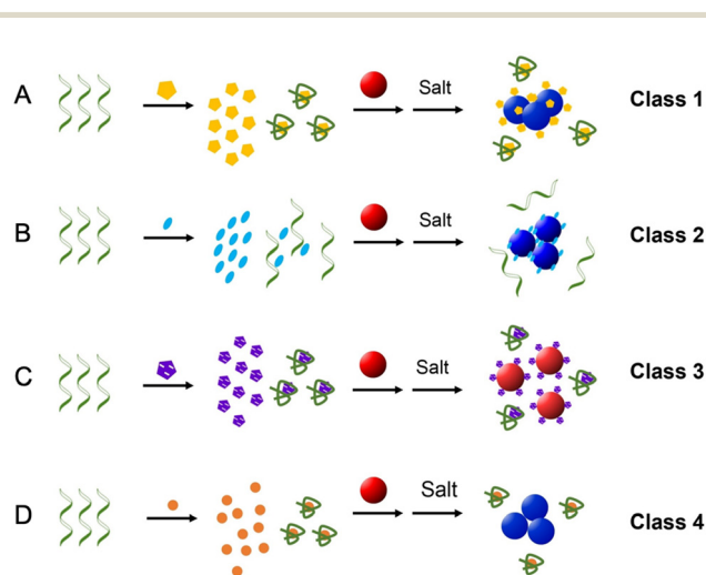
Fig. 7 Categorization of target analytes based on their interaction with AuNPs. (A) Adsorb onto AuNP and lead to destabilization (e.g. dopamine, adenosine), (B) adsorb onto AuNPs with little stabilization or destabilization affects (e.g. As(III)), (C) adsorb onto AuNPs and lead to stabilization (e.g. ATP), and (D) do not adsorb onto AuNPs and have no discernable affects (e.g. \text{K}^+ ). Reproduced from ref. 48 with permission from Chemistry Europe.
