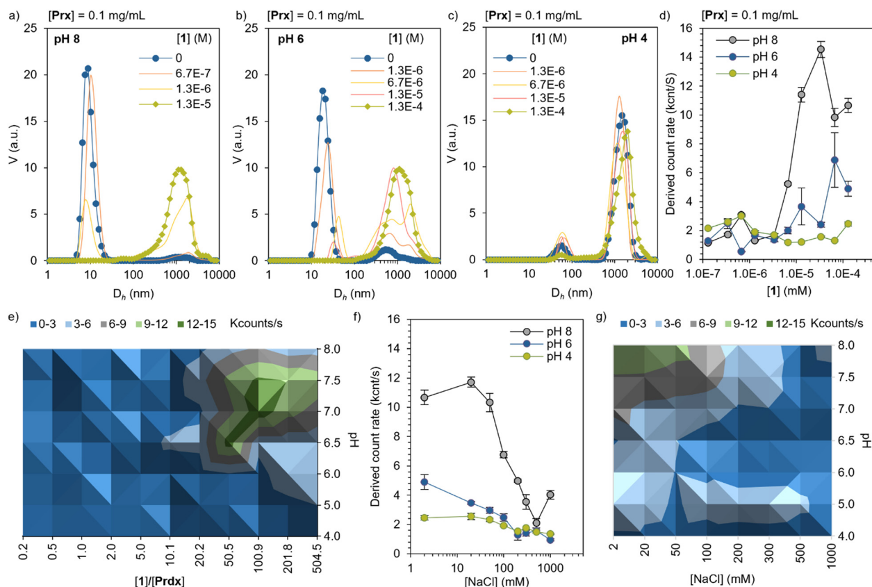
Fig. 2 Self-assembly of Prx – 1 complexes by dynamic light scattering (DLS). Titration of [\mathbf{Prx}] = 0.1 \text{ mg mL}^{-1} with increasing concentrations of 1 , given as volume-averaged size distributions at (a) pH 8, (b) pH 6, and (c) pH 4. (d) Derived count rate, showing a sharp increase upon formation of large complexes. (e) Diagram of complex formation at different pH and 1 ratios. (f) Complex disassembly upon increase of the ionic strength of the media, achieved by NaCl concentration. (g) Phase diagram of disassembly at different pH and NaCl concentration.
