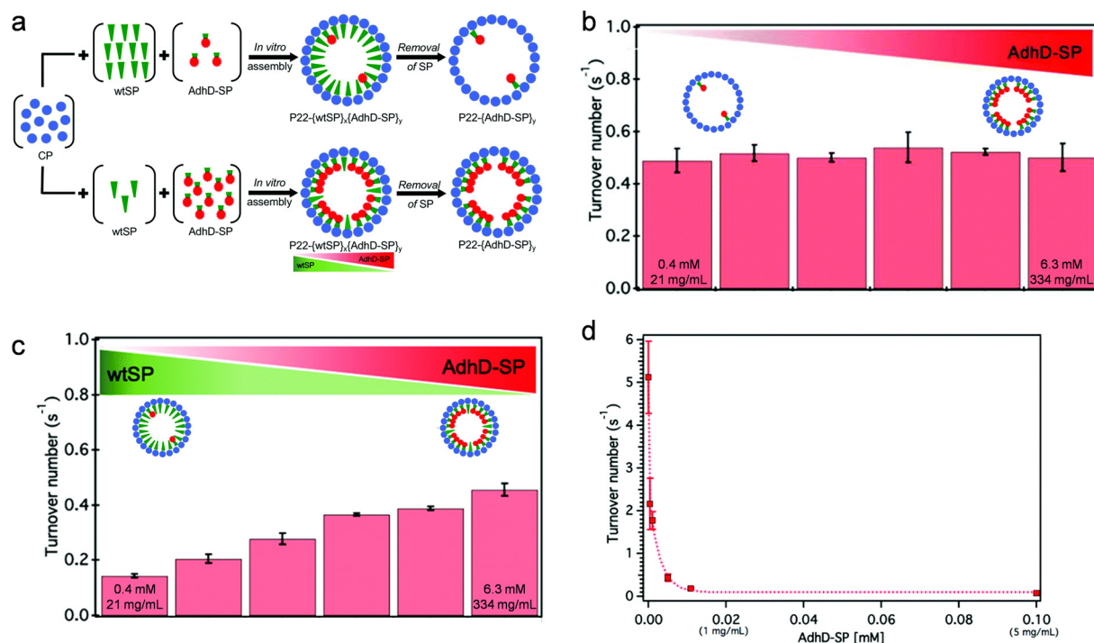
Fig. 2 Crowding and confinement effects on the catalytic activity of alcohol dehydrogenase D (AdhD) inside P22 VLPs. (a) In vitro assembly allows controlled loading of AdhD inside P22 VLPs by co-encapsulation of wild-type scaffold protein (wtSP), which can be removed after particle formation. (b) Self crowding does not have an effect on AdhD activity. (c) wtSP as an inert, non-self crowding agent changes the catalytic activity of AdhD. The extreme local concentrations of AdhD inside the VLPs are labeled in (b) and (c). (d) Activity of free (unencapsulated) AdhD at different concentrations. Reproduced from ref. 26 with permission from the Royal Society of Chemistry.
