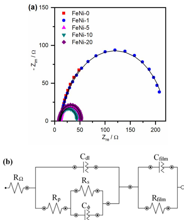
Fig. 6 (a) Nyquist plots for pristine and iron-incorporated nickel hydroxide films measured at 1.52 V vs. RHE in an alkaline medium (1.0 M NaOH) and (b) equivalent circuit employed for fitting the Nyquist plots.
