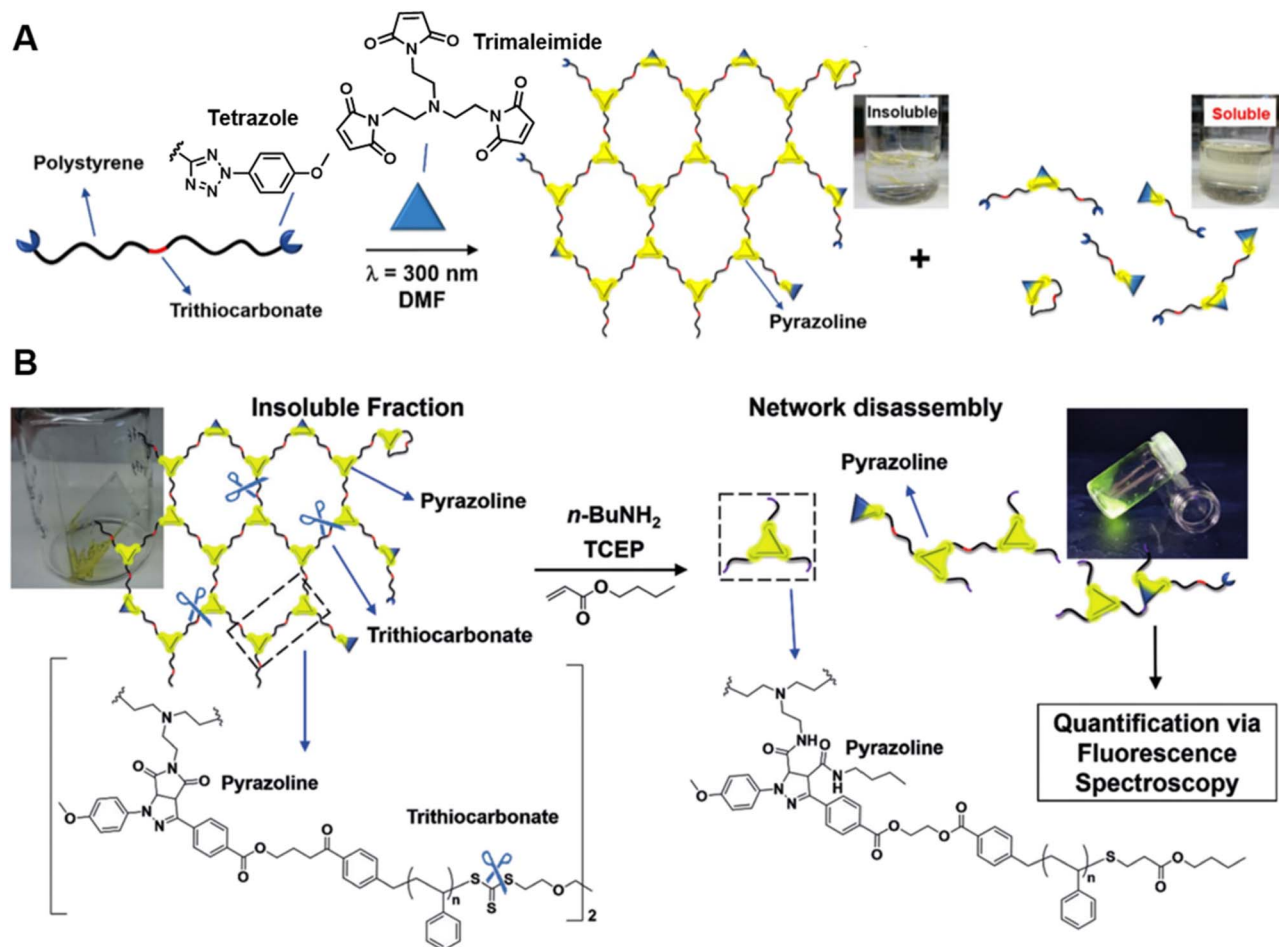
Fig. 7 (A) UV-induced NITEC crosslinking reaction between tetrazole chain-ends and trithialimide cross-linkers, forming insoluble and soluble fractions. (B) Network disassembly via aminolysis. Determining the concentration of pyrazoline after aminolysis via fluorescence spectroscopy allows to quantify the number crosslinking points within the former network. Reproduced from ref. 191 with permission from Wiley, copyright 2018.
