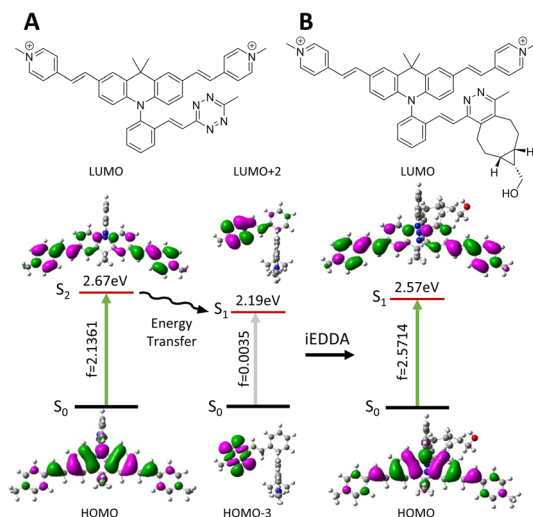
Fig. 5 Molecular structures, optimized geometries, corresponding oscillator strength ( f ) and dominating frontier molecular orbitals involved during these transitions of (A) AcTri-ovi and (B) Clicked AcTri-ovi.
