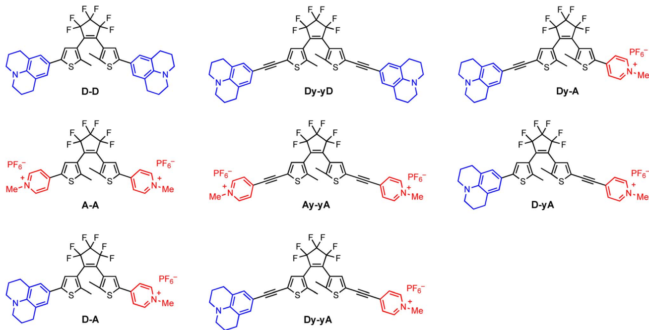
Fig. 1 Structures of the open-form DTEs synthesized, bearing donor–donor, acceptor–acceptor or donor–acceptor substitution patterns. Electron donor and acceptor are julolidine (blue) and N -methylpyridinium (red), respectively. D, A, y and – represent the donor, the acceptor, the alkyne, and the central DTE core, respectively.
