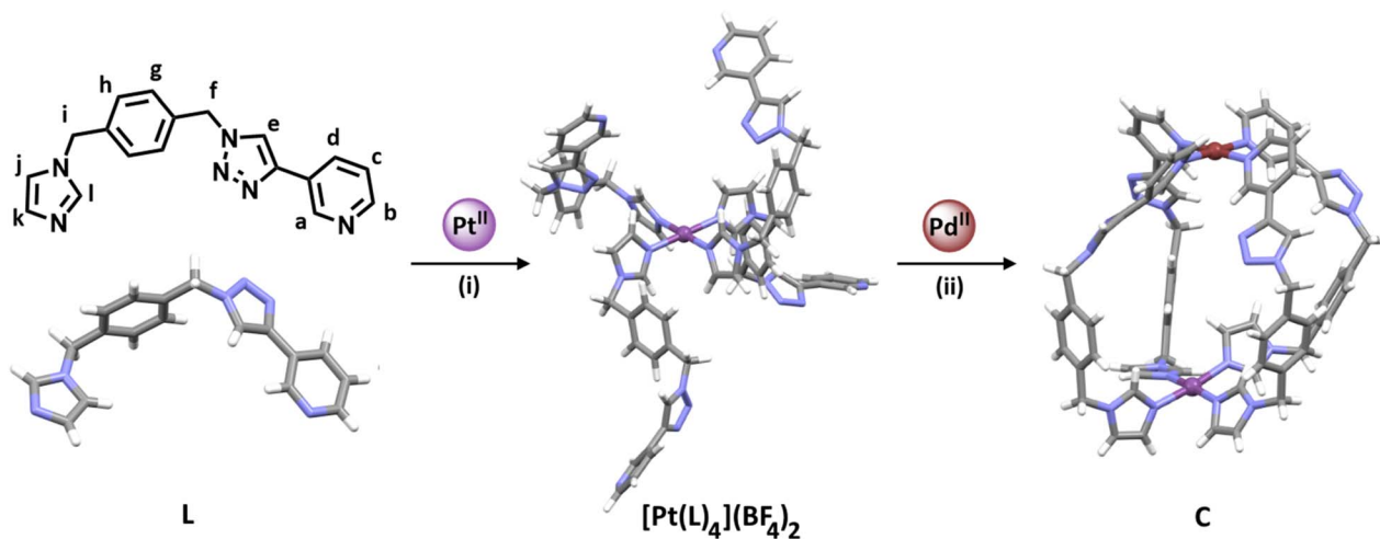
Scheme 1 Synthesis of the platinum(II) complex [Pt(L)_4](BF_4)_2 , and the heterobimetallic low-symmetry cage (C): (i) L (4.1 eq.), AgBF_4 (2.2 eq.), and [Pt(DMSO)_2Cl_2] (1 eq.), d_6 -DMSO, 60 °C, 7 days. (ii) [Pt(L)_4](BF_4)_2 (1 eq.), [Pd(CH_3CN)_4](BF_4)_2 (1 eq.), CD_3CN , RT, 10 min ( [L] = 21.1 mM, [Pt(L)_4](BF_4)_2 = 5.27 mM). The stick model (MMFF) of [Pt(L)_4](BF_4)_2 was generated using SPARTAN'18. 66 Stick models of L and C are the molecular structures determined by X-ray diffraction analysis. Colours: Pd II brick, Pt II purple, N periwinkle blue, C grey, H white. Solvent molecules and counterions omitted for clarity.
