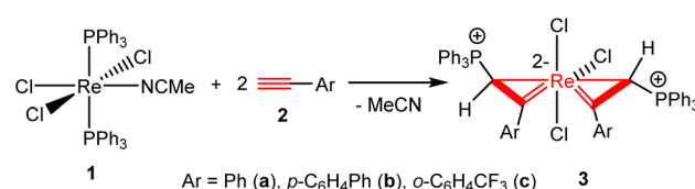
Scheme 2 Syntheses of spiro bi(metallacycloprop-1-ene) complexes 3a–c .
