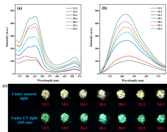
Fig. 1 (a) The PL excitation and (b) emission spectra, and (c) photographs of g-C 3 N 4 -Ph synthesized using melamine and quinazoline-2,4(1 H ,3 H )-dione at molar ratios 12 : 1, 14 : 1, 16 : 1, 18 : 1, 20 : 1, 22 : 1 and 24 : 1, respectively. \lambda_{\text{ex}} = 326 nm, \lambda_{\text{em}} = 508 nm.
