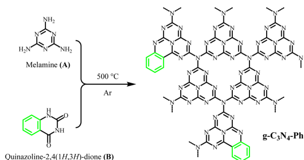
Scheme 1 The synthesis of g-C 3 N 4 -Ph. Molar ratios A : B = x : 1 ( x = 12, 14, 16, 18, 20, 22, and 24).
