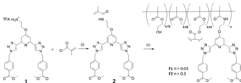
Scheme 1 Synthesis and structure of monomer 2 , formed from ligand 1 , and the two polymeric films F1 and F2 . Reagents and conditions: (i) \text{NEt}_3 , \text{CH}_2\text{Cl}_2 (ii) 80^\circ\text{C} 6 hours. F1 (0.03 wt%) and F2 (0.3 wt%), respectively. Pictures show the films formed before and after being hydrated.
