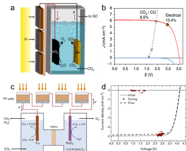
Fig. 11 CO 2 reduction catalysts for PV-EC devices. (a) Schematic of the device combining photovoltaics with an electrochemical cell. (b) J - V curves of three series-connected perovskite solar cells overlaid with the matched J - V characteristic of the CO 2 -reduction and oxygen-evolution electrodes. Reproduced from ref. 197. Copyright 2015 Nature publishing group. (c) Schematic of the light-driven electrochemical device for reduction of CO 2 to CH 4 . (d) J - V curves of 4 series-connected perovskite solar cells before, during, and after 510 nm light-driven CO 2 reduction. Reproduced from ref. 198. Copyright 2019 Cell Press.
