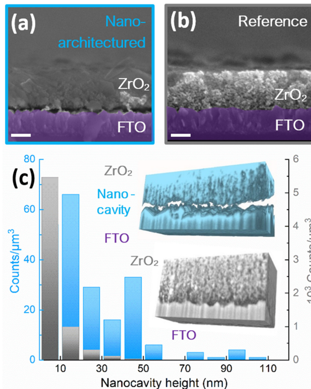
Fig. 2 Cross-sectional scanning electron microscopy (SEM) images of (a) the nano-architected layer of \text{ZrO}_2 and (b) the reference layer of \text{ZrO}_2 . Scale bars – 500 \text{ nm} . (c) Distribution of the cavity height in the nano-architected (blue) and reference (grey) samples, obtained from 3D-nanotomography using focused ion-beam (FIB) ablation.
