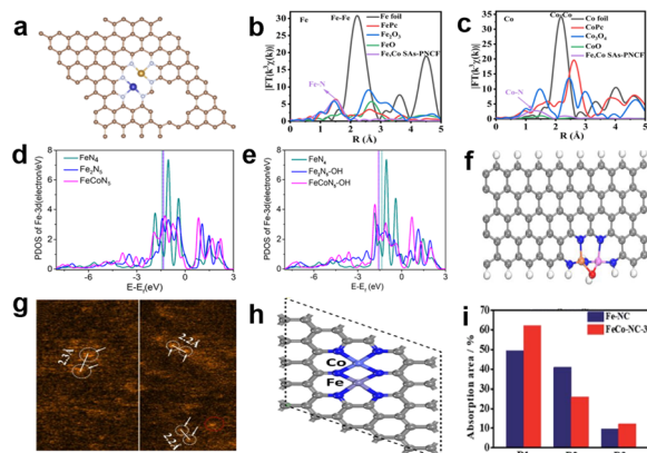
Fig. 15 (a) The schematic structure of Fe, Co SAs-PNCF. 111 FT-EXAFS spectra of (b) Fe K-edge and (c) Co K-edge. 111 Fe 3d PDOS (d) before and (e) after absorption of OH*. 15 (f) The structure of \text{FeCoN}_5\text{-OH} site. 15 (g) AC HAADF-STEM images of \text{FeCoN}_5/\text{C} . 15 (h) The main active site structure of \text{FeCo-NC-3} . 113 (i) The content of three Fe moieties which comes from the analysis of Fe Mössbauer spectroscopy. 113
