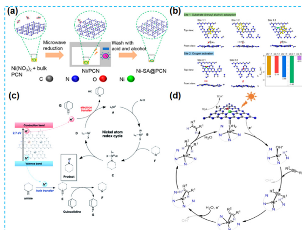
Fig. 19 (a) Diagrammatic illustration of the preparation procedure of Ni-SA@PCN. (b) Theoretical calculations for the absorption of benzyl alcohol (yellow) and the activation of \text{O}_2 (red) on PCN based photocatalysts associated with the corresponding absorption energy ( \Delta E_{\text{ads}} ) on different binding sites. 84 (c) The proposed mechanism of photoredox C–N coupling on NiSA@CN. 85 (d) The proposed visible-light-driven semihydrogenation mechanism mediated by single-atom Ni. Here TEA quenched the photogenerated hole on CN, making electrons available for the formation of active \text{Ni}^+ . 86
