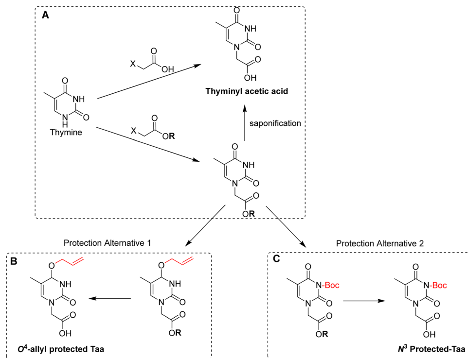
Scheme 13 (A) Two basic routes for the synthesis of thymine acetic acid; (B) synthesis of O 4 -allyl-protected thymine acetic acid and (C) synthesis of N 3 -Boc-protected thymine acetic acid.
