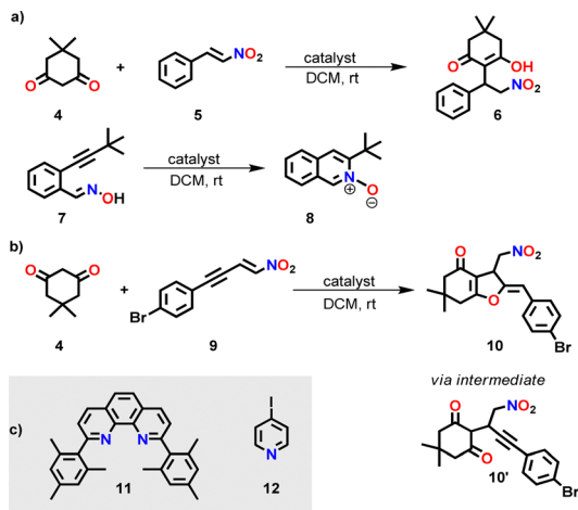
Scheme 2 (a) Parallel one-pot base-catalyzed Michael addition and silver(i)-catalyzed cyclization. For catalyst(s), see Tables 1 and 2. (b) Sequential Michael addition/hydroalkoxylation reaction (for mechanism, see ESI,† Scheme S4). 17 (c) Further ligands used in this study.
