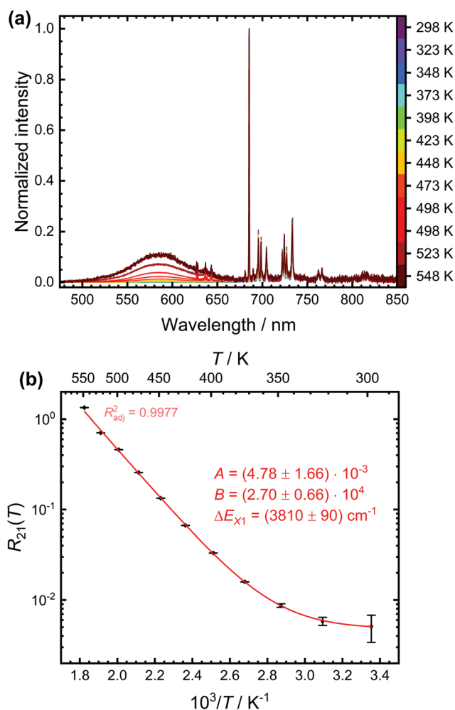
Fig. 4 (a) Temperature-dependent emission spectra of \text{SrBa}_4\text{O}_7:0.5\% \text{Sm}^{2+} ( \lambda_{\text{ex}} = 423 \text{ nm} ) normalized to the intensity of the most intense ^5\text{D}_0 \rightarrow ^7\text{F}_0 transition. The peaks on the top of the broad 4\text{f}^55\text{d}^1 \rightarrow 4\text{f}^6 -based emission band stem from the ^5\text{D}_1 \rightarrow ^7\text{F}_J ( J = 0, 1, 2 )-related emission. (b) Data (black points) and least-squares fit (red line) according to eqn (4) of the temperature-dependent luminescence intensity ratio between the 4\text{f}^55\text{d}^1 \rightarrow 4\text{f}^6 - and ^5\text{D}_0 \rightarrow ^7\text{F}_J -based emission. The fitting parameters and the adjusted (squared) correlation coefficient indicating the quality of the fit is given as well.
