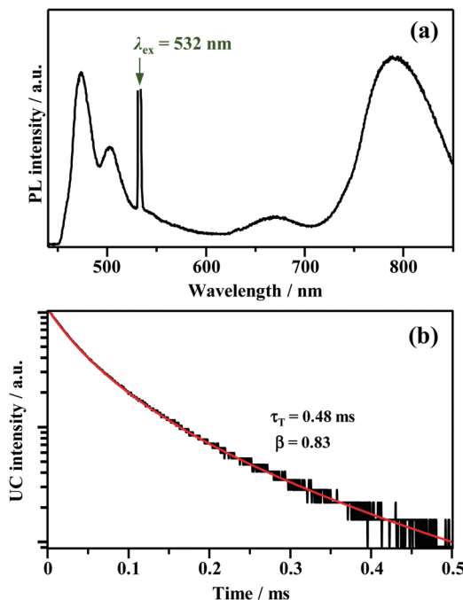
Fig. 4 (a) PL spectrum obtained for the deaerated THF solution of \text{Au}_2\text{Cu}_6 (11 \mu M) and perylene (5 mM), and (b) decay curve of the upconverted emission of perylene obtained by monitoring only the \lambda \leq 492 nm region using short-pass filters. The fitting of the decay curve was performed using eqn (1). The 532 nm-CW laser was used in these measurements. Note that the upconverted emission of perylene was also observed when using a 640 nm-CW laser.
