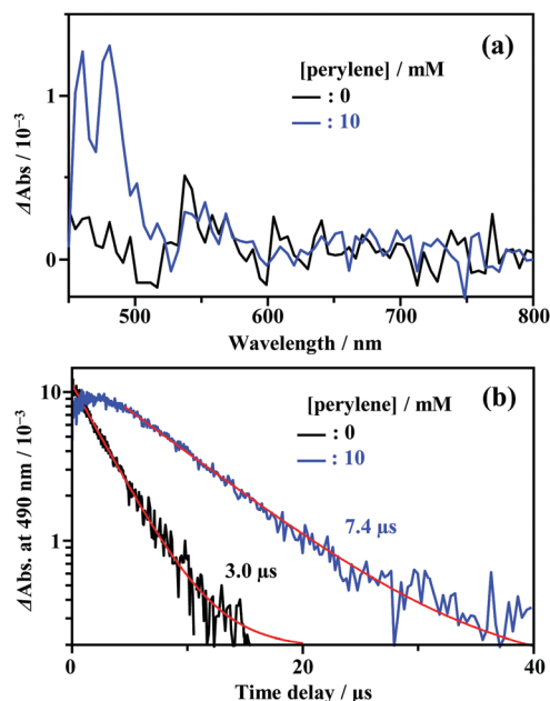
Fig. 3 (a) Transient absorption (TA) spectra at the time delay of 20 \mu s and (b) decay time profiles of the TA signal at 490 nm, measured for \text{Au}_2\text{Cu}_6 (270 \mu M) with 0 and 10 mM perylene in deaerated THF at 298 K (excitation wavelength, \lambda_{\text{ex}} = 532 nm).
