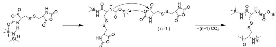
Scheme 2 Typical routes for controlled polymerization of Cys 2 NCA. HMDS: hexamethyl disilamine.
