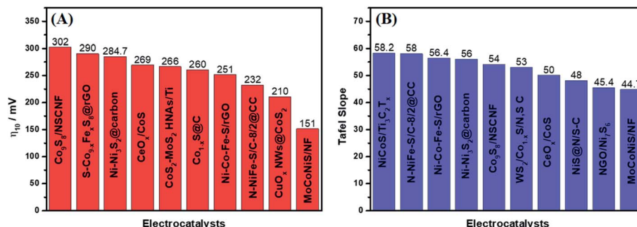
Fig. 24 The top ten sulfide-based electrocatalysts derived from MOFs considering (A) the \eta_{10} overpotential values and (B) the Tafel slopes.
