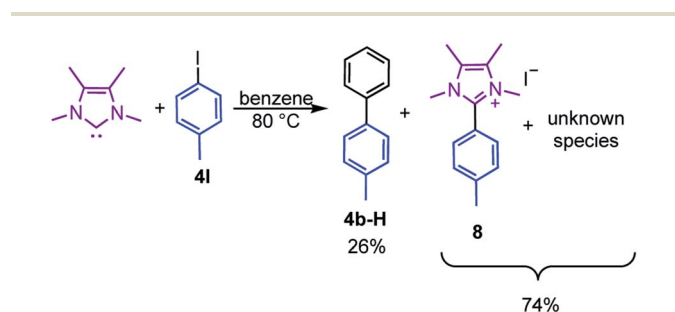
Scheme 4 Reaction of the free NHC \text{Me}_2\text{Im}^{\text{Me}} with 4-iodotoluene 4I at 80 °C forming the C–C coupling product with the solvent 4b-H , the imidazolium salt [4\text{-CH}_3\text{-Ph-Me}_2\text{Im}^{\text{Me}}]^+\text{I}^- 8 , and an unknown compound.
