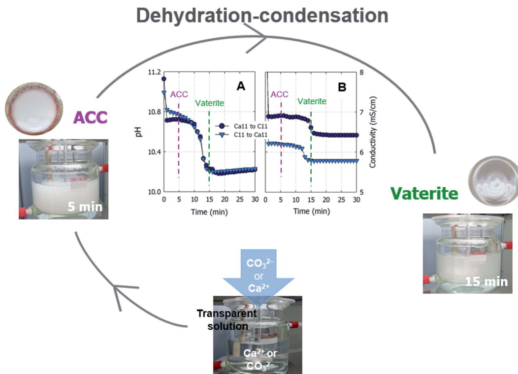
Fig. 3 Possible reaction pathway based on the observation of particles formed over time. Variations of (A) pH and (B) conductivity in solutions with time after the rapid mixing of equal volumes of the 50 mM Ca11/C11. Ca and C represent the calcium chloride and sodium (bi)carbonate solutions, respectively, and the adjacent numbers represent the starting pH values of the individual solutions.
