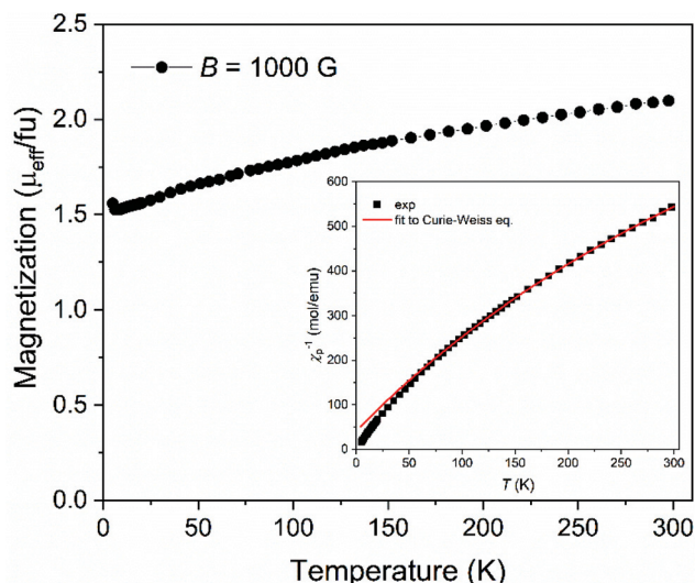
Fig. 1 Magnetic properties of \text{Na}[\text{o}^{57}\text{FESAN}] powder sample: temperature dependence of the magnetization under a magnetic field of 0.1 T. Inset: temperature dependence of the inverse of the magnetic susceptibility. The solid red line is the fit to the Curie–Weiss law of the experimental data (solid square symbols).
