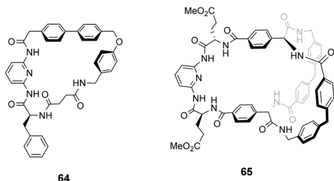
Fig. 24 Macrocyces 64 and 65 .
