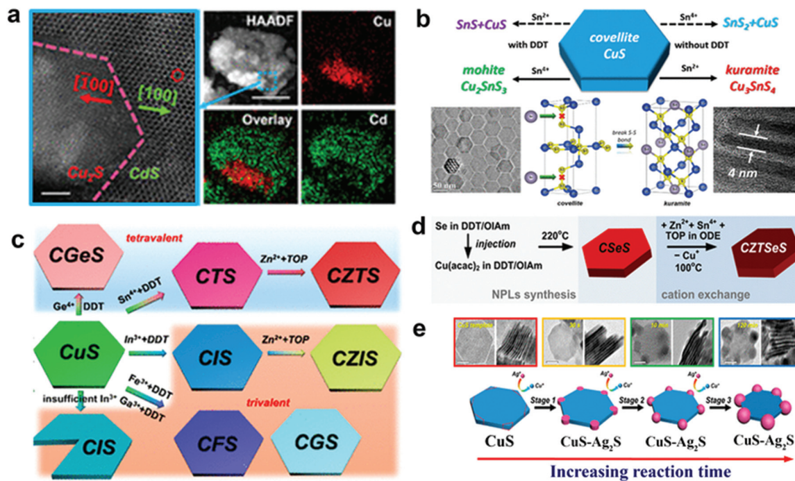
Fig. 2 (a) CE of the covellite CuS template with \text{Cd}^{2+} forming a heterostructure of \text{Cu}_2\text{S}-\text{CdS} ; reproduced from ref. 61 with permission from ACS, copyright 2018; (b) illustration of outcomes from CE of the covellite CuS template with \text{Sn}^{2+} and \text{Sn}^{4+} cations in the presence and absence of dodecanethiol as the reducing agent; reproduced from ref. 37 with permission from ACS, copyright 2017; (c) schematic of the CE product from CuS using tri and tetravalent cations. Reproduced from ref. 61 with permission from ACS, copyright 2018; (d) sequential CE of the \text{Cu}_{2-x}\text{Se}_y\text{S}_{1-y} template forming multi-elemental \text{Cu}_2\text{ZnSnSe}_y\text{S}_{1-y} nanoplates. Reproduced from ref. 96 with permission from ACS, copyright 2014; (e) CE of \text{Ag}^+ on the CuS template leading to segregated \text{Ag}_2\text{S} formation at the corners of CuS nanoplates. Reproduced from ref. 97 with permission from ACS, copyright 2018.
