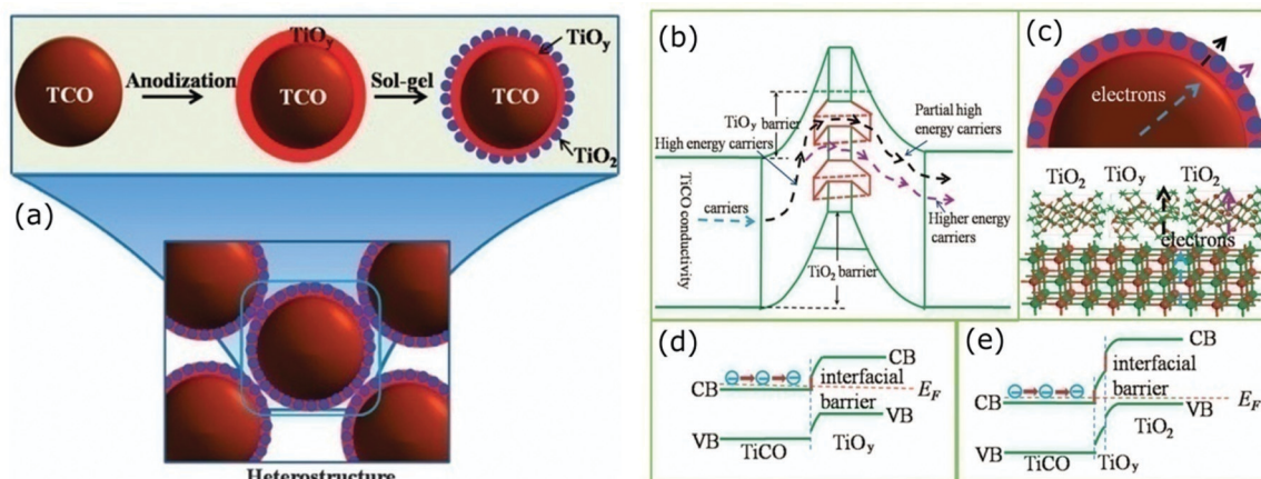
Fig. 7 (a) Schematic illustration of the formation of the \text{Ti}_{1-x}\text{O}_x\text{@TiO}_y\text{-TiO}_2 heterostructures via anodization process. The mechanism of carrier transport through the double-barrier: (b) carrier paths where the first interfacial \text{TiO}_y barrier selectively scatters low-energy carriers and the \text{TiO}_2 barrier further scatters partial high-energy carriers, (c) transport schemes of the carriers in the heterostructures and at the interface, (d) and (e) show the band diagrams of the all-oxide \text{Ti}_{1-x}\text{O}_x\text{@TiO}_y and \text{Ti}_{1-x}\text{O}_x\text{@TiO}_y\text{-TiO}_2 heterostructured interfaces. Reproduced with permission from ref. 110, Copyright 2015 Nature Publishing Group.
