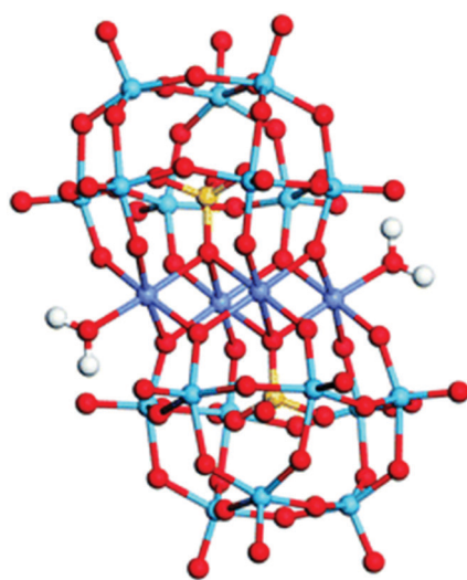
Fig. 133 Structural model of [\text{Ni}_4(\text{H}_2\text{O})_2(\text{SiW}_9\text{O}_{34})_2]^{12-} ( \text{M} = \text{Ni} ; \text{W} : blue, \text{O} : red; \text{S} : yellow; \text{H} : white; \text{M} : dark blue). Reprinted with permission from ref. 1600. Copyright 2012 RSC.
