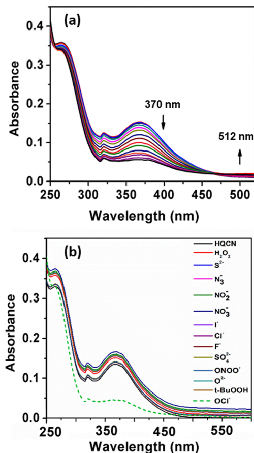
Fig. 2 (a) UV-vis spectra of HQCN ( 10\ \mu\text{M} in \text{CH}_3\text{OH}-\text{H}_2\text{O} ; 1/4 , v/v in the presence of HEPES buffer ( 10\ \text{mM} ) solution at \text{pH} = 7.2 ) upon the gradual addition of \text{OCl}^- (0 to 5 equivalents). Ratiometric spectra of HQCN were observed after the addition of \text{OCl}^- . The absorption peak of HQCN at 370\ \text{nm} gradually decreased and the peak at 512\ \text{nm} gradually increased after the addition of \text{OCl}^- with an isosbestic point at 462\ \text{nm} . (b) UV-vis spectra of HQCN ( 10\ \mu\text{M} in \text{CH}_3\text{OH}-\text{H}_2\text{O} ; 1/4 , v/v in the presence of HEPES buffer ( 10\ \text{mM} ) solution at \text{pH} = 7.2 ) upon addition of different guest analytes (0 to 5 equivalents). Apart from \text{OCl}^- , no significant change was observed upon the addition of the other guest analytes.
