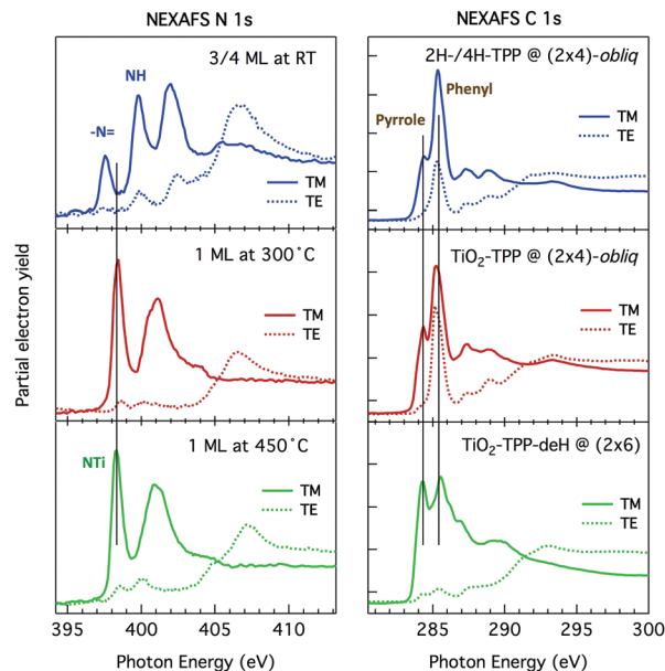
Fig. 17 NEXAFS spectra measured in partial electron yield at the N and C K-edges, left and right panels, respectively, at RT, 300^\circ\text{C} and 450^\circ , corresponding to different molecular species and symmetry phases; spectra measured in TM and TE polarization are represented as full and dotted lines, respectively. The surface was azimuthally oriented to keep the scattering plane along the [001] direction. In this geometry, the TE spectra are measured with the electric field transverse to the rows, where the molecules display a slightly larger intensity of \pi -symmetry resonances than along the rows, hence yielding the maximum tilt angle/molecular distortion in any chemical state. Adapted from ref. 49 with permission from the Royal Society of Chemistry, Copyright 2017.
