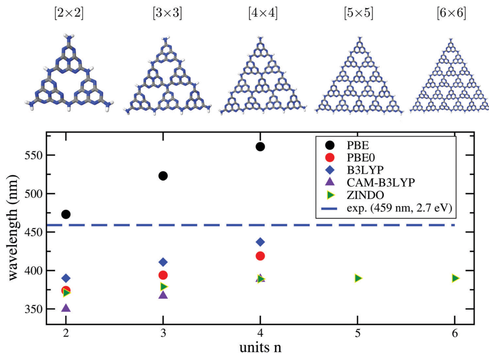
Fig. 7 Upper part: Different [ n \times n ] cluster models used in this work to characterize the optical properties of g-C 3 N 4 . As in Fig. 3, cluster structures were taken from the periodic calculations of ref. 16, and only the N–H distances were reoptimized, with PBE+D3/6-311G**. Lower panel: Wavelengths for the lowest-energy TD-DFT excitations obtained by TD-DFT/6-311G** (DFT = PBE, PBE0, B3LYP, CAM-B3LYP) and by the semiempirical ZINDO method, for various cluster sizes. The experimental gap (2.7 eV, 459 nm) is shown for comparison as a horizontal line.
