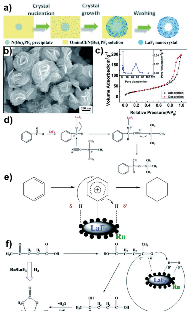
Fig. 5 (a) A scheme for the formation of hollow mesoporous \text{ReF}_3 (Re = La, Nd, or Y) nanocrystals. (b) SEM image of mesoporous \text{LaF}_3 nanocrystals. (c) Nitrogen adsorption and desorption isotherms of mesoporous \text{LaF}_3 nanocrystals shown in (b) (pore-size distribution is included in the inset). (d) Proposed reaction mechanism for the cyanosilylation reaction catalysed by \text{LaF}_3 . (e) Proposed reaction mechanism for the benzene hydrogenation to cyclohexane using the co-catalyst \text{Ru/LaF}_3 . (f) Proposed reaction mechanism for levulinic acid (LA) hydrogenation to \gamma -valerolactone using the co-catalyst \text{Ru/LaF}_3 . 95 Reprinted with permission from ref. 95. Copyright 2015, Royal Society of Chemistry.
