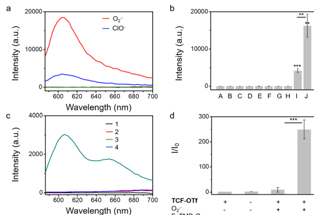
Fig. 1 (a and b) Selectivity of TCF-OTf (10 μM) towards a range of ROS and other substances existing in bacteria, after reacting for 2 h. A, probe only; B, ONOO - (100 equiv.); C, HO • (100 equiv.); D, 1 O 2 (100 equiv.); E, H 2 O 2 (100 equiv.); F, GSH (100 equiv.); G, Fe 3+ (100 equiv.); H, ROO • (100 equiv.); I, ClO - (100 equiv.); and J, O 2 •- (10 equiv.). (c and d) Fluorescence emission spectrum of TCF-OTf (10 μM) (c) and the corresponding change in fluorescence (d) in the absence or presence of O 2 •- and FeTMPyP (100 μM) in PBS buffer solution (10% DMSO, pH = 7.40). 1, TCF-OTf; 2, FeTMPyP; 3, TCF-OTf + O 2 •- (pos.); and 4, TCF-OTf + O 2 •- and FeTMPyP (neg.). **P < 0.01, ***P < 0.001. λ ex = 560 nm, λ em = 606 nm.
