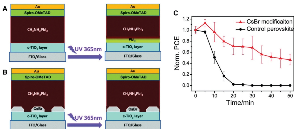
Fig. 9 Schematic depicting a PSC containing a typical compact \text{TiO}_2 /perovskite interface before and after UV exposure (A). A PSC containing cesium bromide ( \text{CsBr} ) interfacial modifiers before and after UV exposure (B). Normalized PCE for \text{CsBr} modified (initial PCE of 15.3%) and control (initial PCE of 11.3%) devices as a function of time under 100 \text{ mW cm}^{-2} UV light (C). Reproduced with permission from ref. 52. Copyright 2016 The Royal Society of Chemistry.
