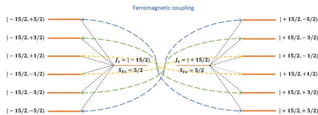
Fig. 14 Energy splitting of the lowest manifold arising from the exchange coupling between a strong anisotropic lanthanide ion (e.g., Dy^{III} ) and a transition metal ion (e.g., Fe^{III} ) in weak ZFS. Here orange lines are energy levels, colored lines with arrows indicates the most preferred relaxation channel for population at corresponding energy level. Lines with the same color are expected to have the same transition rate. Dominant path is the competition between different colored lines. Effective blocking barrier can thus range from the height of the fourth to the sixth energy levels depending on the specific system and temperature.
