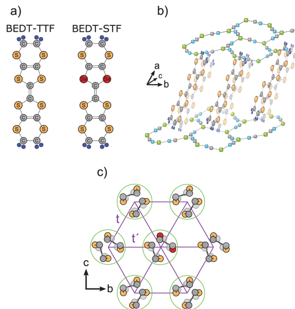
Fig. 2 (a) Organic donor molecules bis-(ethylenedithio)-tetrathiafulvalene, called BEDT-TTF and bis-(ethylenedithio)-diseleniundithiafulvalene, abbreviated BEDT-STF. In the latter case, two sulfur atoms of the inner rings are replaced by selenium. (b) The crystal structure contains dimers of the donor molecules forming layers in the bc -plane which are separated by the Cu 2 (CN) 3 anion sheets. (c) The dimers are arranged in a triangular pattern with transfer integrals t'/t = 0.83 close to complete frustration. The STF-substitution, which is randomly distributed in space, leads to a local extension of the transfer integrals due to the larger molecular orbitals.
