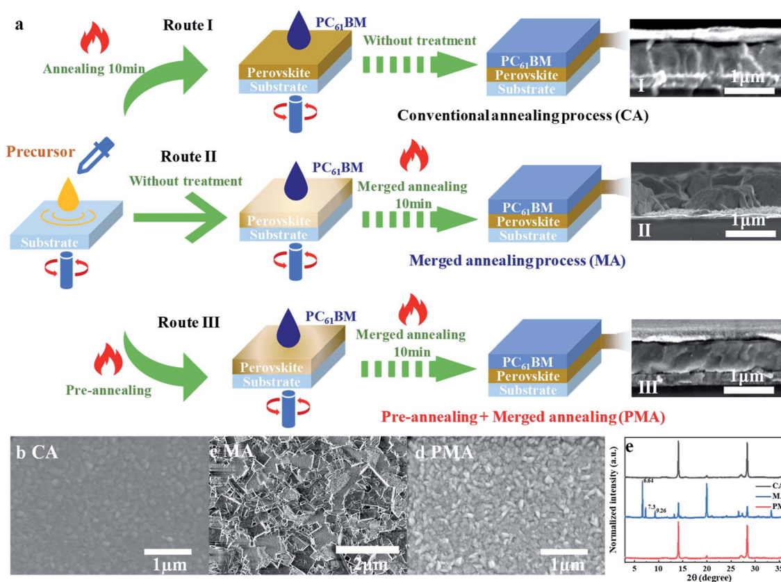
Fig. 1 (a) Schematic illustration of three fabrication processes for a PC_{61}BM coated (3AMP)(MA_{0.75}FA_{0.25})_3Pb_4I_{13} film and the cross-sectional SEM images for the corresponding films. Top-view SEM images of (3AMP)(MA_{0.75}FA_{0.25})_3Pb_4I_{13} films fabricated by CA (b), MA (c) and PMA (d) processes. (e) X-ray diffraction (XRD) patterns of perovskite films fabricated by various methods.
