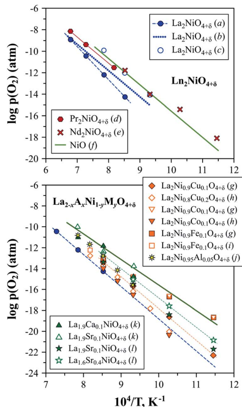
Fig. 5 Low- p\text{O}_2 stability boundaries of \text{Ln}_2\text{NiO}_{4+\delta} and \text{La}_{2-x}\text{A}_x\text{Ni}_{1-y}\text{M}_y\text{O}_{4+\delta} nickelates. Literature sources: (a) ref. 212, (b) ref. 211, (c) ref. 63, (d) ref. 222, (e) ref. 58, (f) ref. 223, (g) ref. 120, (h) ref. 214, (i) ref. 121, (j) ref. 189, (k) ref. 153 and (l) ref. 56.
