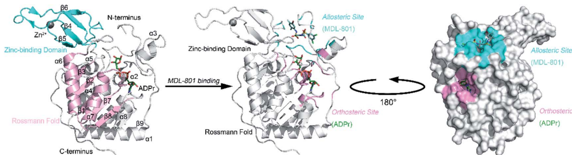
Fig. 1 Structural overview of Sirt6 with major secondary structural elements and functional domains specified. The zinc-binding domain (ZBD) and Rossmann fold (PDB ID: 5X16) are shown in cyan and pink, respectively (left panel). Structural overview of the allosteric activator (MDL-801)-bound Sirt6 with highlighted ADPr orthosteric site (pink) and MDL-801 allosteric site (cyan) (PDB ID: 5Y2F) (middle). Structural overview of MDL-801-bound Sirt6 showing the distal binding pocket of MDL-801 to orthosteric ADPr pocket. This confirmed its allosteric nature (PDB ID: 5Y2F) (right).
