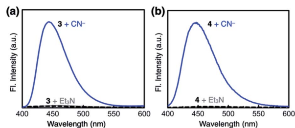
Fig. 7 Emission spectra ( \lambda_{\text{exc}} = 343 \text{ nm} ) of (a) 3 (0.100 mM) prior to (black dashed lines) and after treatment with \text{NaCN} (25 equiv., blue line) or \text{Et}_3\text{N} (25 equiv., gray line), and (b) 4 (0.100 mM) prior to (black dashed lines) and after treatment with \text{NaCN} (25 equiv., blue line) or \text{Et}_3\text{N} (25 equiv., gray line) in DMSO at T = 298 \text{ K} .
