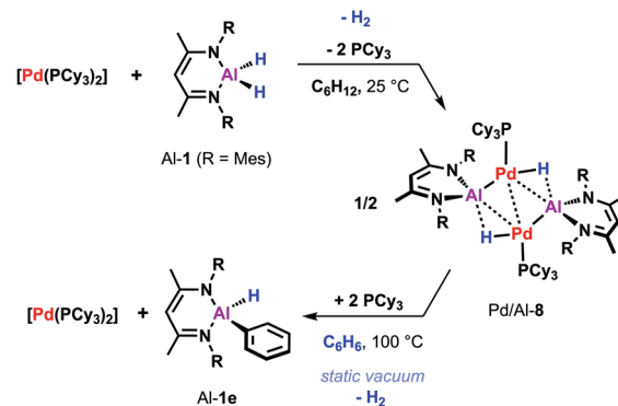
Scheme 7 (a) Pd-catalysed C–H aluminatation of benzene with Al-1. (b) Stoichiometric reactivity of [\text{Pd}(\text{PCy}_3)_2] with Al-1.
