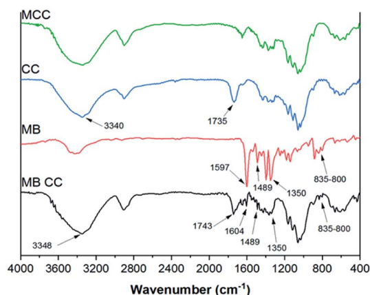
Fig. 1 FT-IR spectra of microcrystalline cellulose (MCC, green), cellulose citrate (CC, blue), methylene blue (MB, red), methylene blue adsorbed on cellulose citrate (MB-CC, black).
